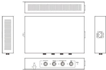
Size (mm): 280(L)X175(W)X53(H)
